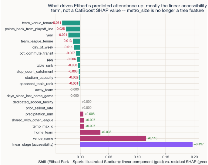
Fig. 2. TreeSHAP decomposition of the predicted shift in log(attendance) from Sports Illustrated Stadium to Etihad Park, averaged across 54 paired synthetic rows. The linear accessibility term (purple) is the single largest contributor, ahead of venue and home-team recognition; every other residual feature contributes close to zero.
